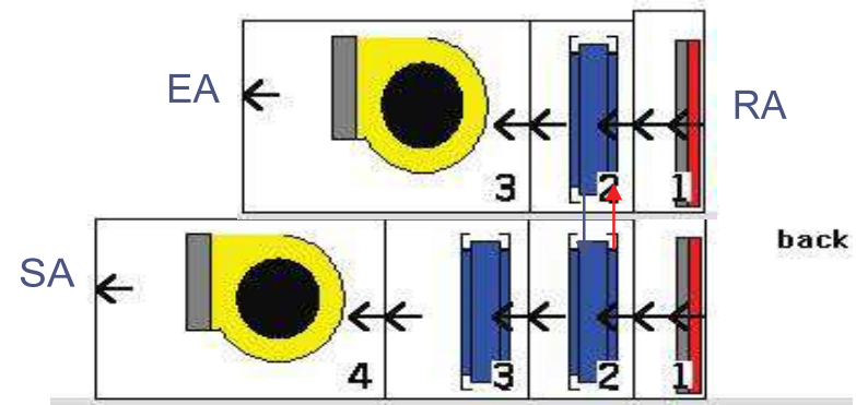
Typical AHU Configuration
